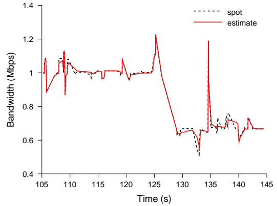
Figure 6: Error-Based Filter Example
