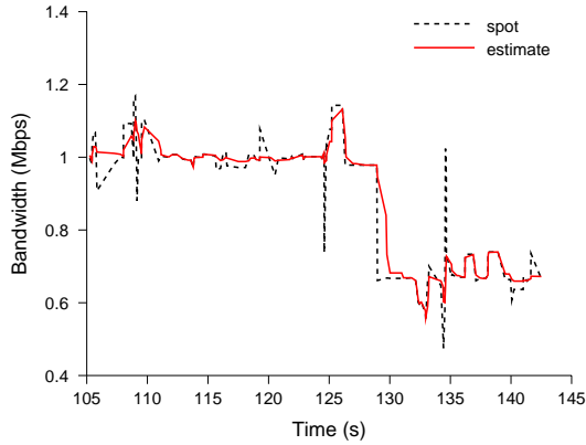
Figure 5: Stability Filter Example
