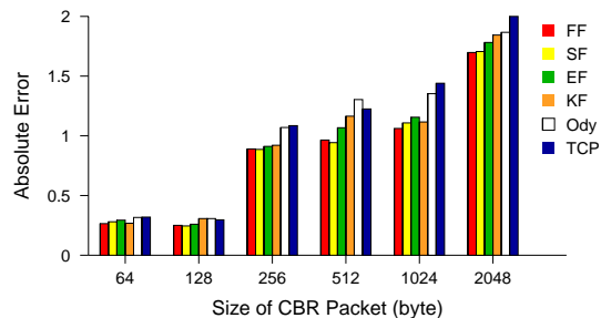
This figure shows the filters' ability to correctly predict round trip times in a large ad hoc network. The X axis lists the packet sizes of background traffic. The Y axis shows the average error produced by each filter's estimates, in seconds; lower errors are better. In general, increased background traffic leads to less accurate predictions. At relatively low levels of background traffic, each filter is comparable. As background traffic increases, the Flip-Flop and Stability filters begin to show advantages.
