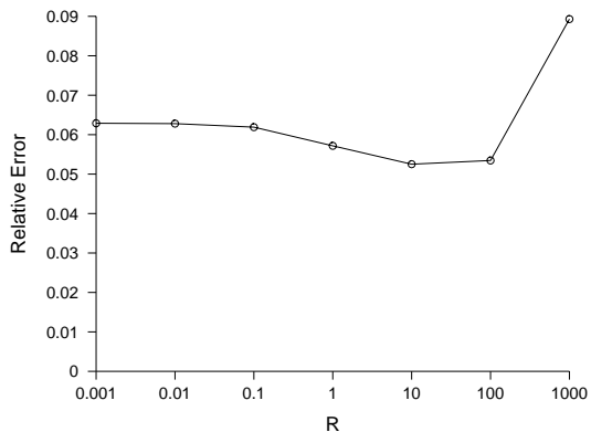
This figure shows relative error of Kalman filter with different \mathbf{R} values under the simple ad hoc network simulation described in Section 5.5.
