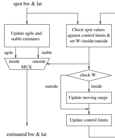
Figure 3: Flip-Flop Filter
